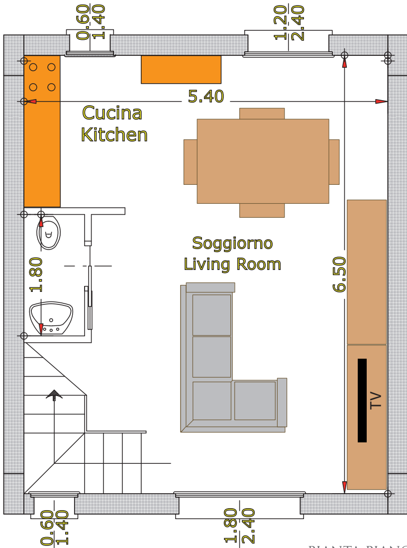
PIANTA PIANO TERRA PLANT GROUND FLOOR
