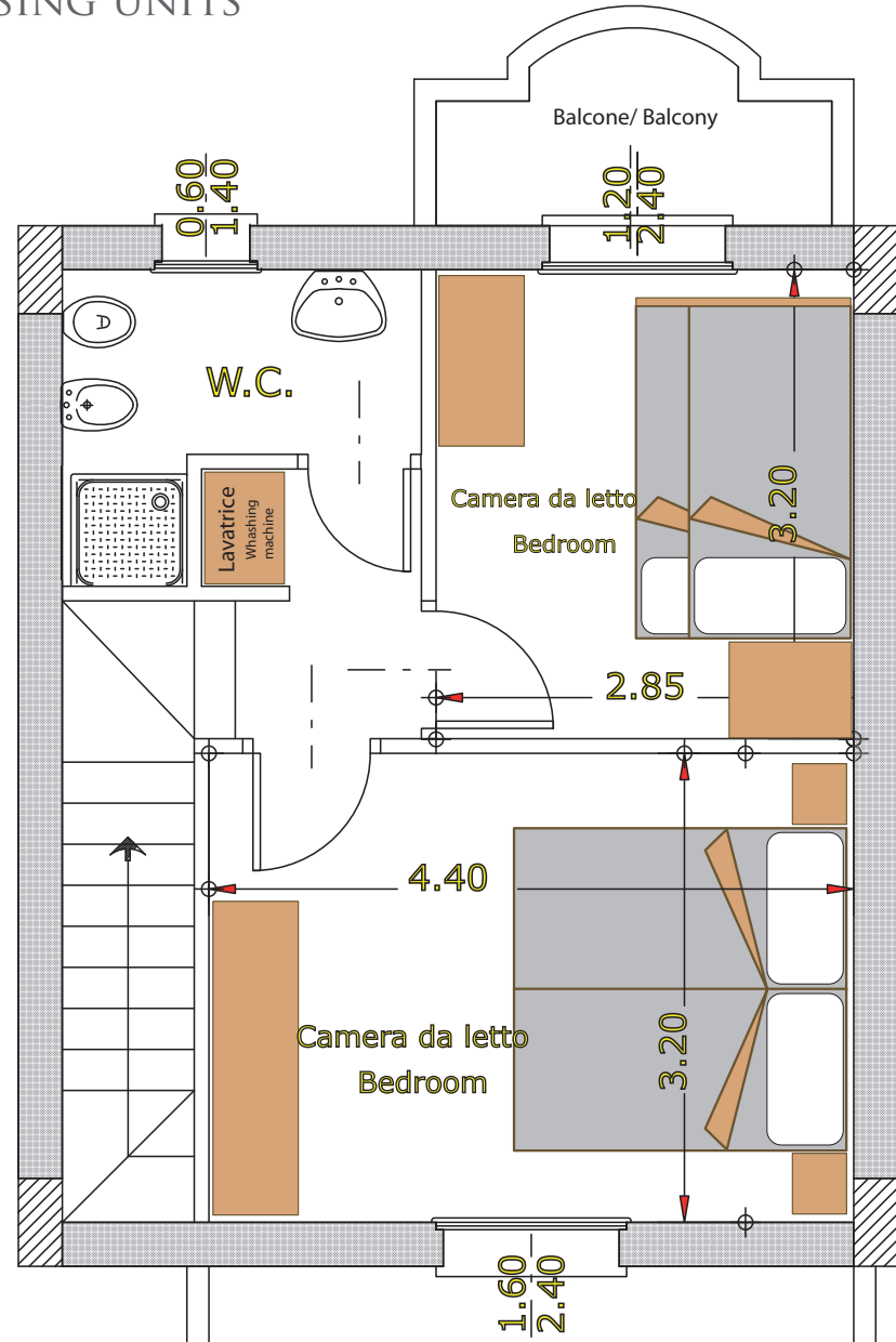
PIANTA PIANO PRIMO PLANT FIRST FLOOR
